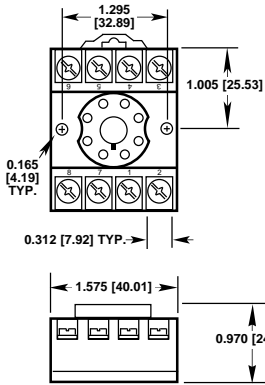
API 008 8-Pin Socket 600 V Rating
