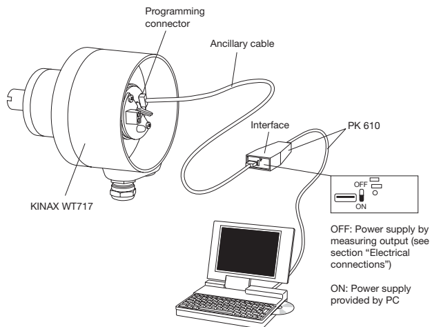
Fig. 4. Example of the set-up for programming a KINAX WT 717 without the power supply. For this case the switch on the interface must be set to «ON».
