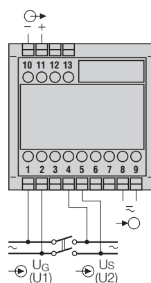
Fig. 2. Power supply to terminals 8 and 9.
