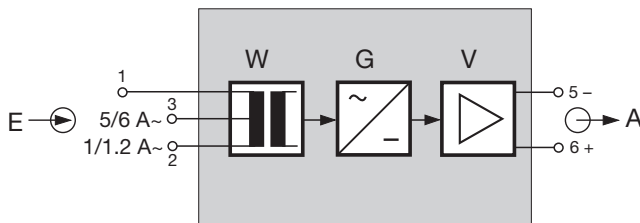
Fig. 2. Block diagram.
