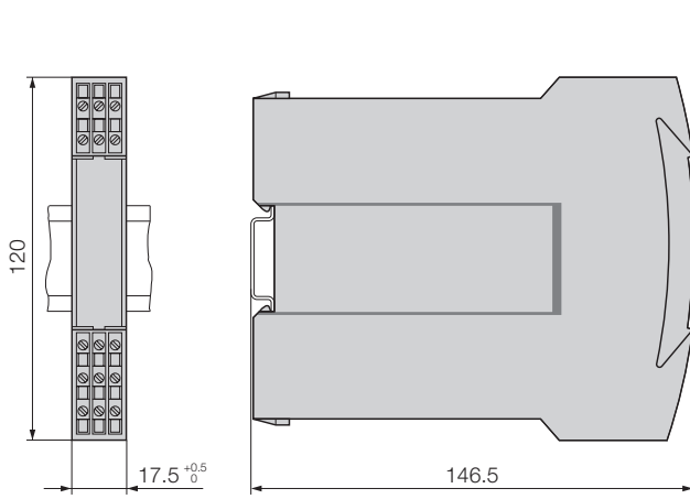
Fig. 4. SINEAX TV 808 in housing S17 clipped onto a top-hat rail (35 × 15 mm or 35 × 7.5 mm, acc. to EN 50 022).
