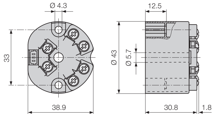
Fig. 5. SINEAX VK 616-72/74, input/output electrically isolated.
