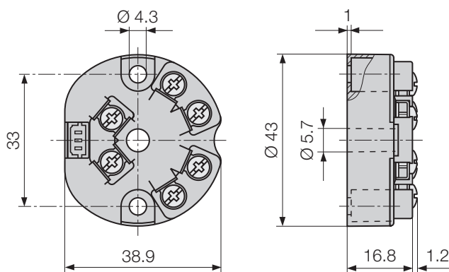
Fig. 4. SINEAX VK 616-71/73, input/output not electrically isolated.
