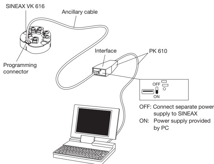
Fig. 3. Example of the set-up for programming a SINEAX VK 616 without the power supply. For this case the switch on the interface must be set to "ON".
