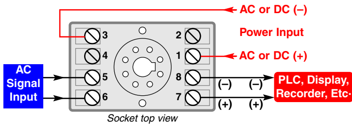
API 6010 G typical output wiring
