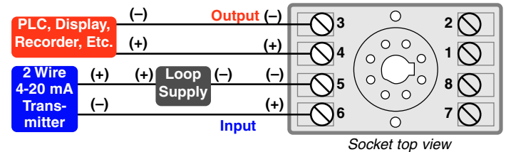
API LPI-1 typical wiring
