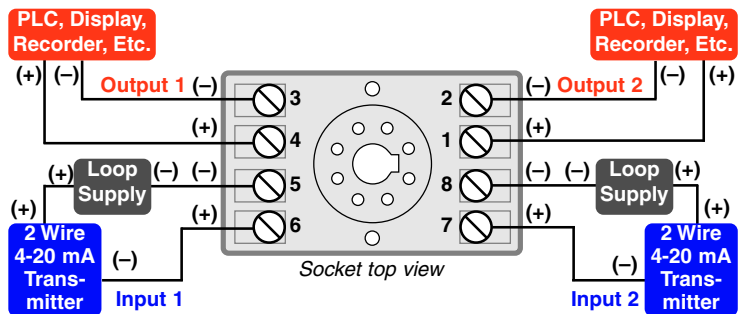
API LPI-2 typical wiring
