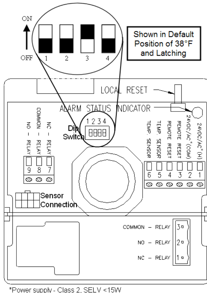
Figure 2 – Setpoint Adjustment Diagram
