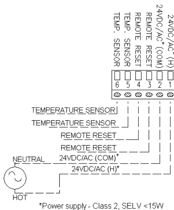
Figure 5 – Diagram of Electrical Connections
