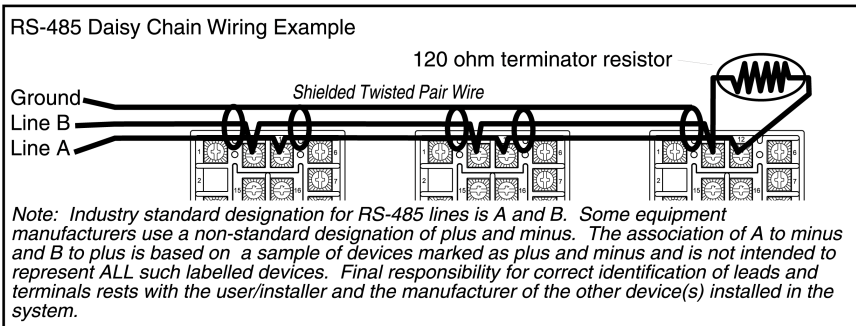
View of rear of instrument showing wiring terminals.
