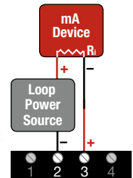
Current Sinking Output
