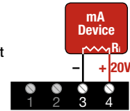
Current Sourcing Output
