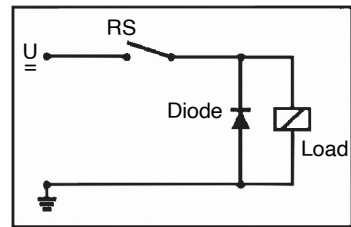
Figure 4: Protection at DC and inductive load by recovery diode
